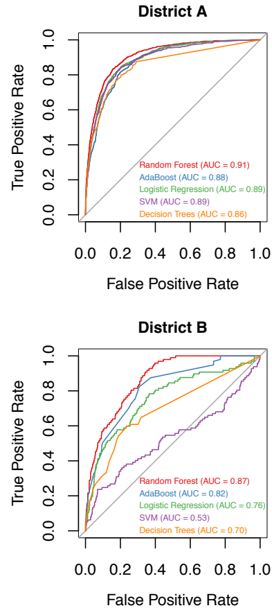
Figure 1: ROC Curves
